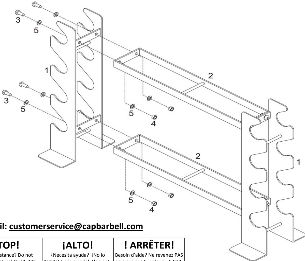
M8 Washer (5) Arandela/Rondelle
